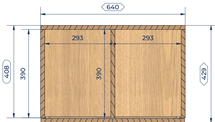
B-B (1:10)
