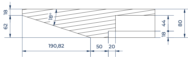
H-H (1:5)
